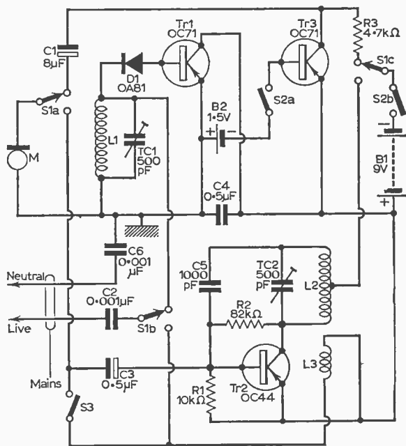
Fig. 1: Complete circuit of the wireless intercom.
