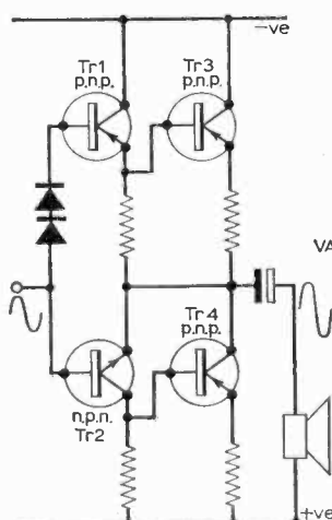
Fig. 3: Complementary driver stage feeding two pnp transistors Tr3 and Tr4 in the output stage.
