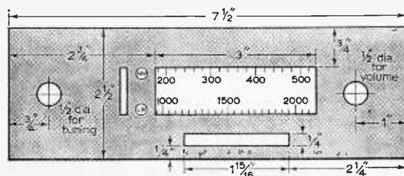
Fig. 6: Layout and drilling details for the front panel.
