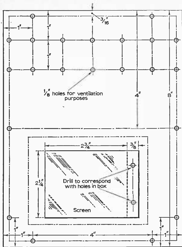
Fig. 7: Details of the baseplate and lower insert, screen for crystals.
