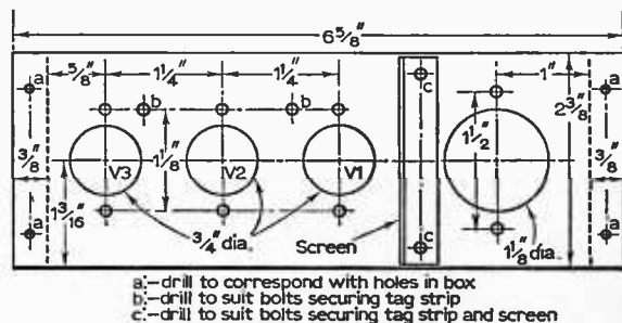
Fig. 8: Details of the chassis-panel.
