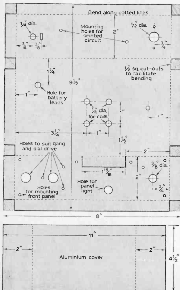
▼ Fig. 4: Layout and drilling dimensions of the chassis-cum-case.
