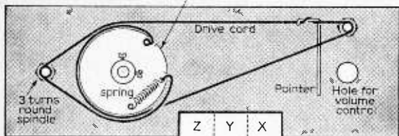
Fig. 5: Details of the positioning of the dial drive for the tuning capacitor.
