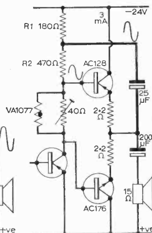
Fig. 4: Complementary output stage driven by a bootstrapped single transistor driver stage. Heavy line is bootstrap connection.
